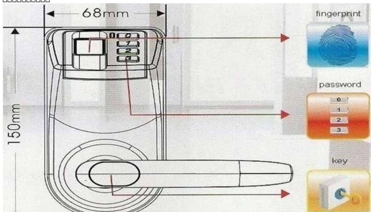
Figure 1: Product Dimensions
